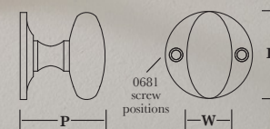
9169 - Cabinet Knob & Rosette
