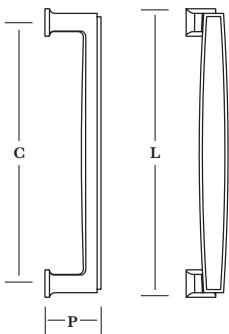
9512 Cabinet / Appliance Pull
