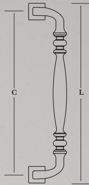
6999 Cabinet /Appliance Pull Shown in Hand Burnished Brass
