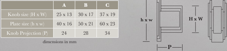
0669 - Cabinet Knob and Plate - Square Edge design Shown in Pearl Nickel
